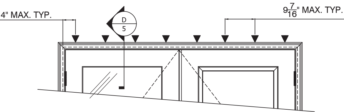
XX HEAD EXTERIOR VIEW
