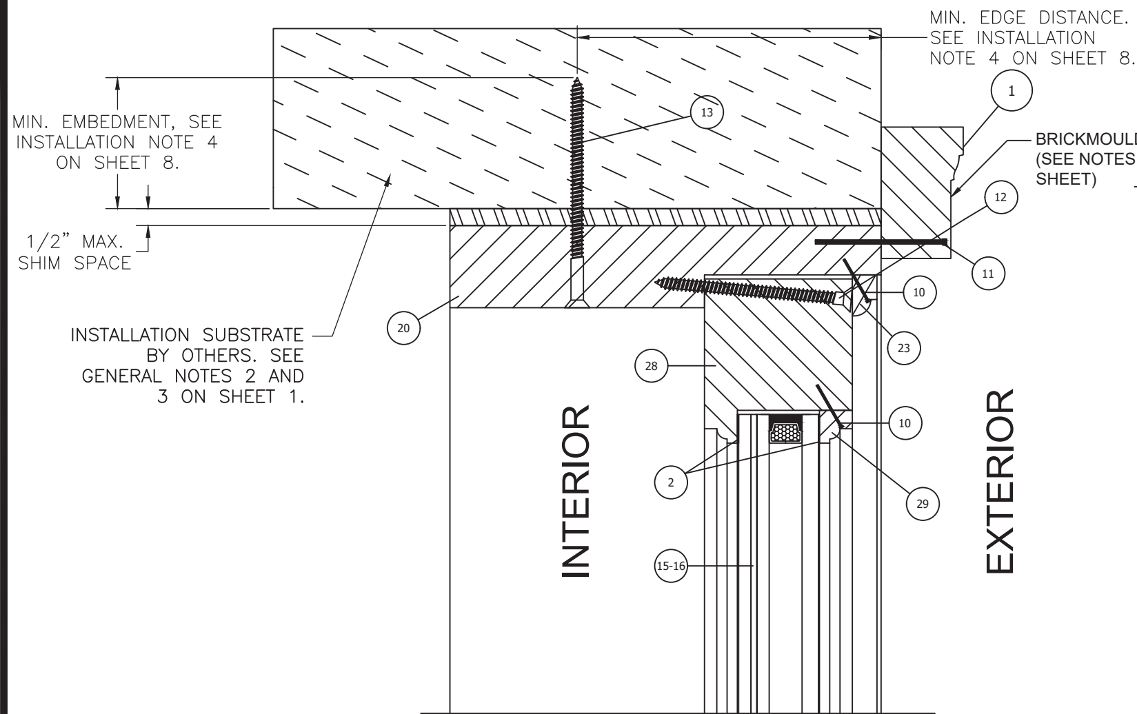
VERTICAL CROSS SECTION TRANSOM HEAD WOOD FRAMING, 2X WOOD BUCK OR CONCRETE/MASONRY SUBSTRATES APPROVED. GLAZED PANEL SHOWN.
