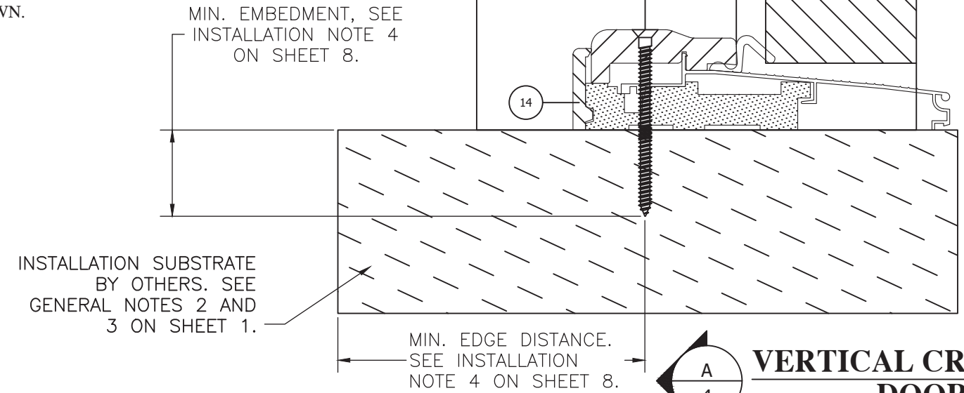
VERTICAL CROSS SECTION TRANSOM HEAD WOOD FRAMING, 2X WOOD BUCK OR CONCRETE/MASONRY SUBSTRATES APPROVED. GLAZED PANEL SHOWN.
